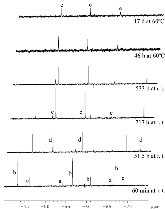
Figure 2. 19 F NMR spectroscopic data for the stepwise hydrodefluorination of perfluorocyclopentene. Temperatures (°C) and allowed reaction times for the various spectra are listed in the right margin. (a = octafluorocyclopentene; b = 1H-heptafluorocyclopentene; c = 1H,2H-hexafluorocyclopentene; d = 1H,2H,3H-pentafluorocyclopentene; e = 6 ).
