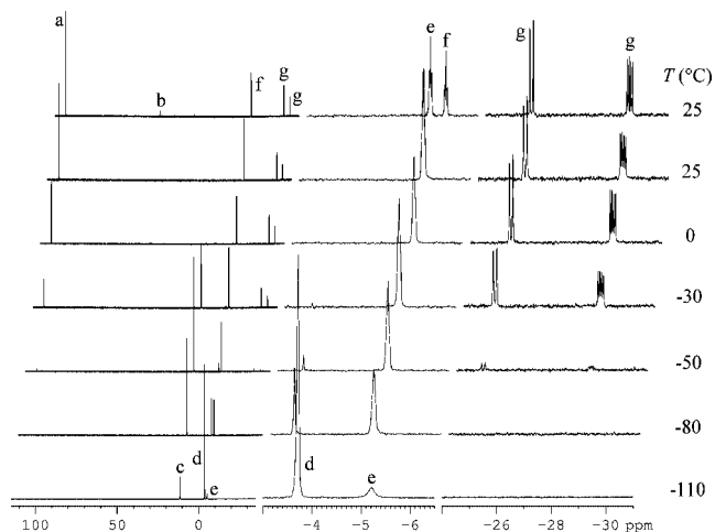
Figure 3. Variable-temperature ^{19}\text{F} NMR spectroscopic data for the reaction of 3,3,3-trifluoropropene with 1 . The temperatures (°C) corresponding to the various spectra are given in the right margin. Regions of interest are expanded for clarity. (a = 2 , b = 3 , c = 7 , d = 3,3,3-trifluoropropene, e = 8 , f = 1,1,1-trifluoropropane, g = 1,1-difluoropropene).
