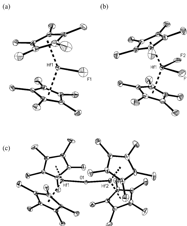
Figure 1. ORTEP diagrams of: a) 2 ; b) 3 ; and c) 4 . Ellipsoids are drawn at the 50% probability level. Hydrogen atoms are omitted for clarity. The fluoride ligand in 2 is disordered over two sites.
